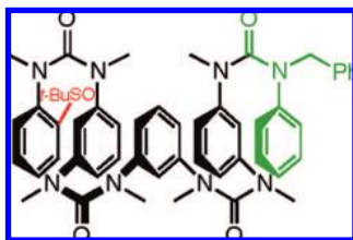
Figure 7. Stacked, helical conformation proposed for 20c .
