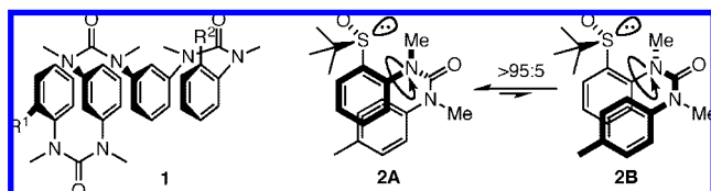
Figure 3. Conformational preferences in ureas.
