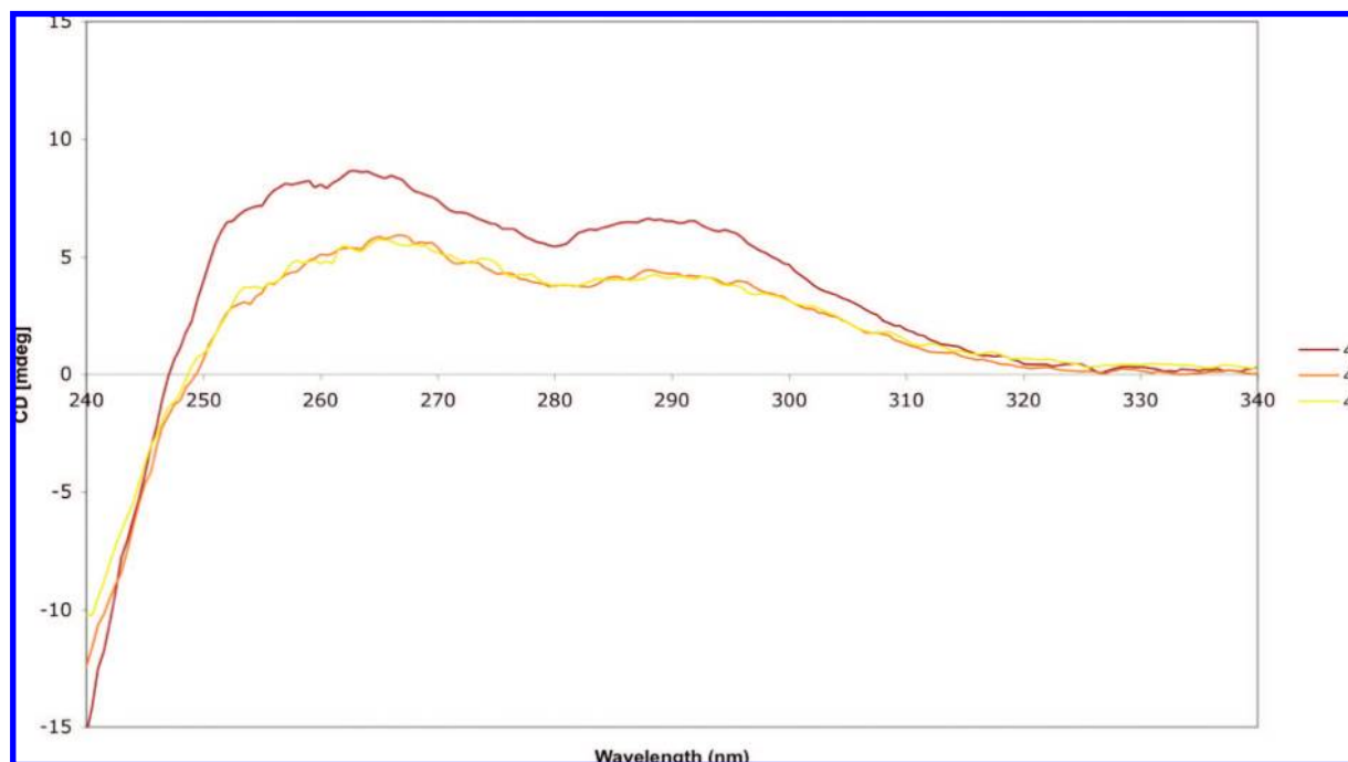
Figure 5. CD spectra of 4a–c.
