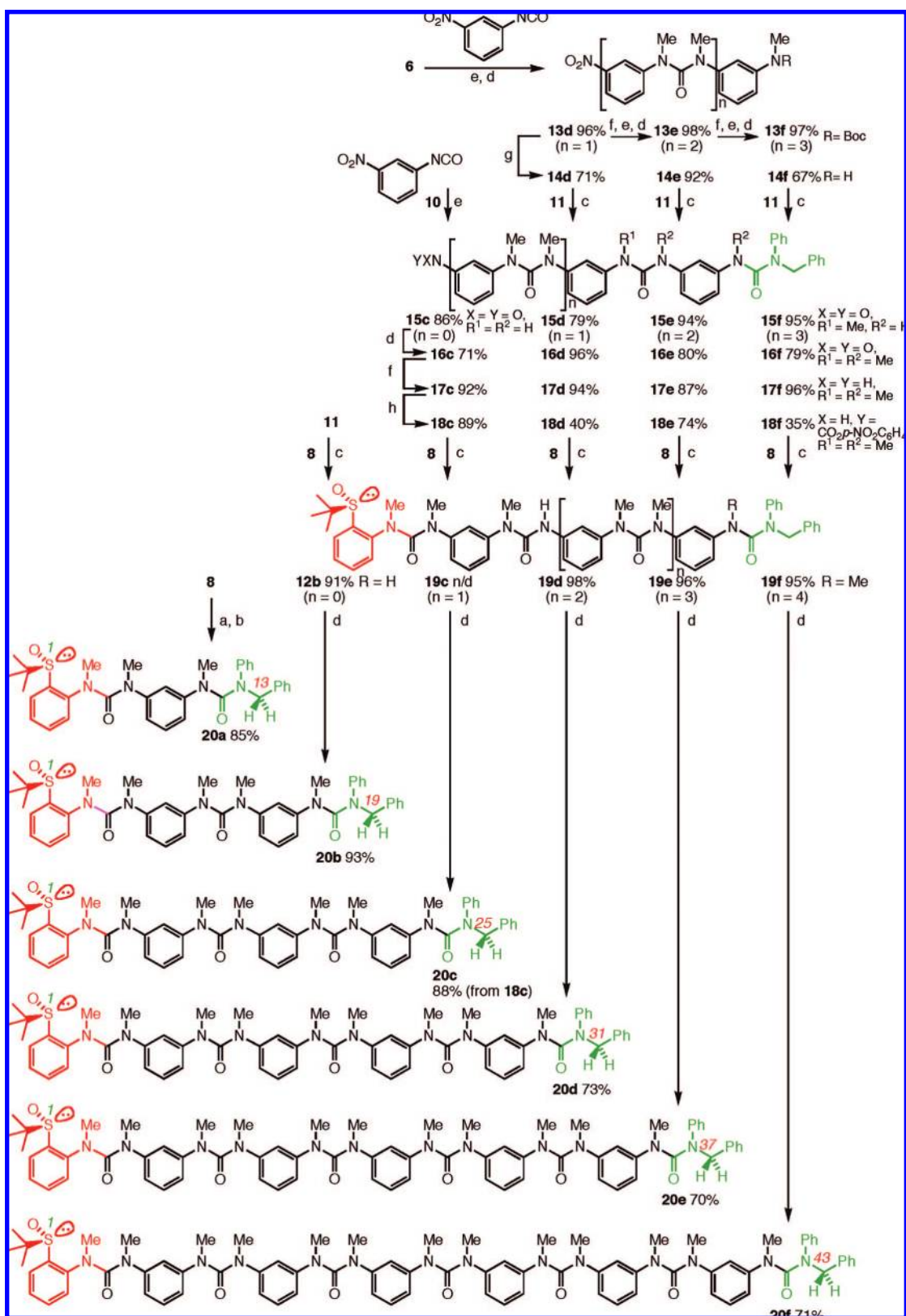
Scheme 4. Construction of Oligoureas a
