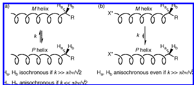
Figure 1. Fast and slow interconversion of enantiomeric and diastereoisomeric helices.
