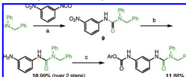
Scheme 3. Synthesis of the N -Benzyl Terminus a
