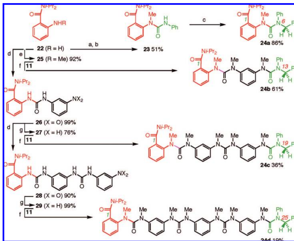
Scheme 5. Synthesis of Amidoureas a
