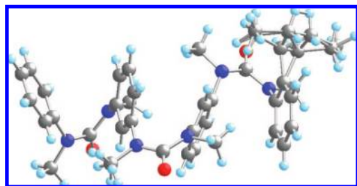
Figure 2. X-ray crystal structure of 1 [ R^1 = H , R^2 = s\text{-Bu} ]. 36
