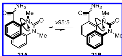
Figure 4. Conformation of an amido urea.
