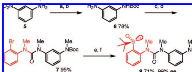
Scheme 2. Synthesis of the Sulfoxide Terminus a
